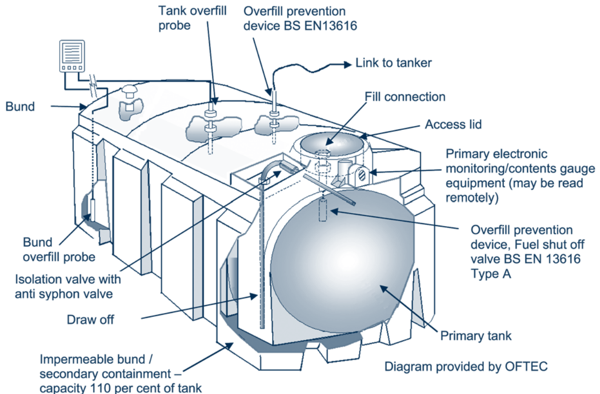
Figure 2. Example of integrally bundled tank (could be constructed of metal or polyethylene and may not be this shape and design)
